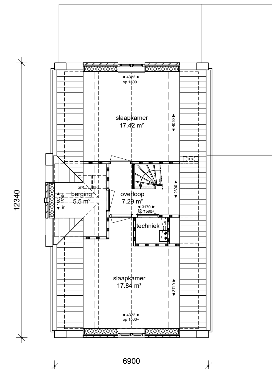
zolder
