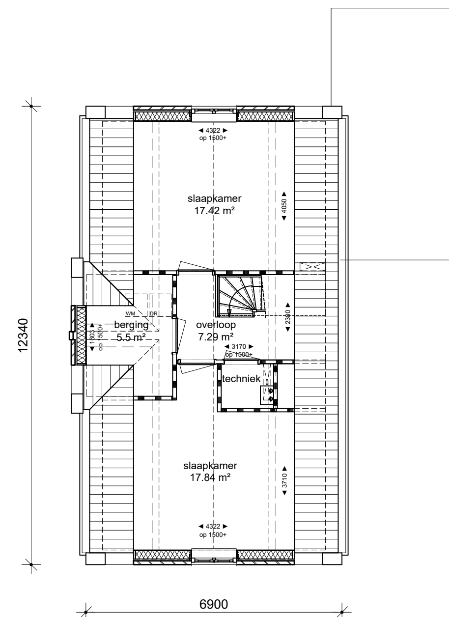
zolder
