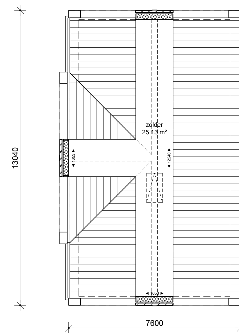
zolder
