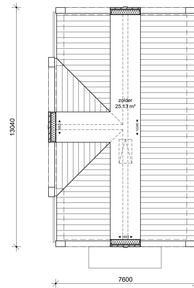
zolder
