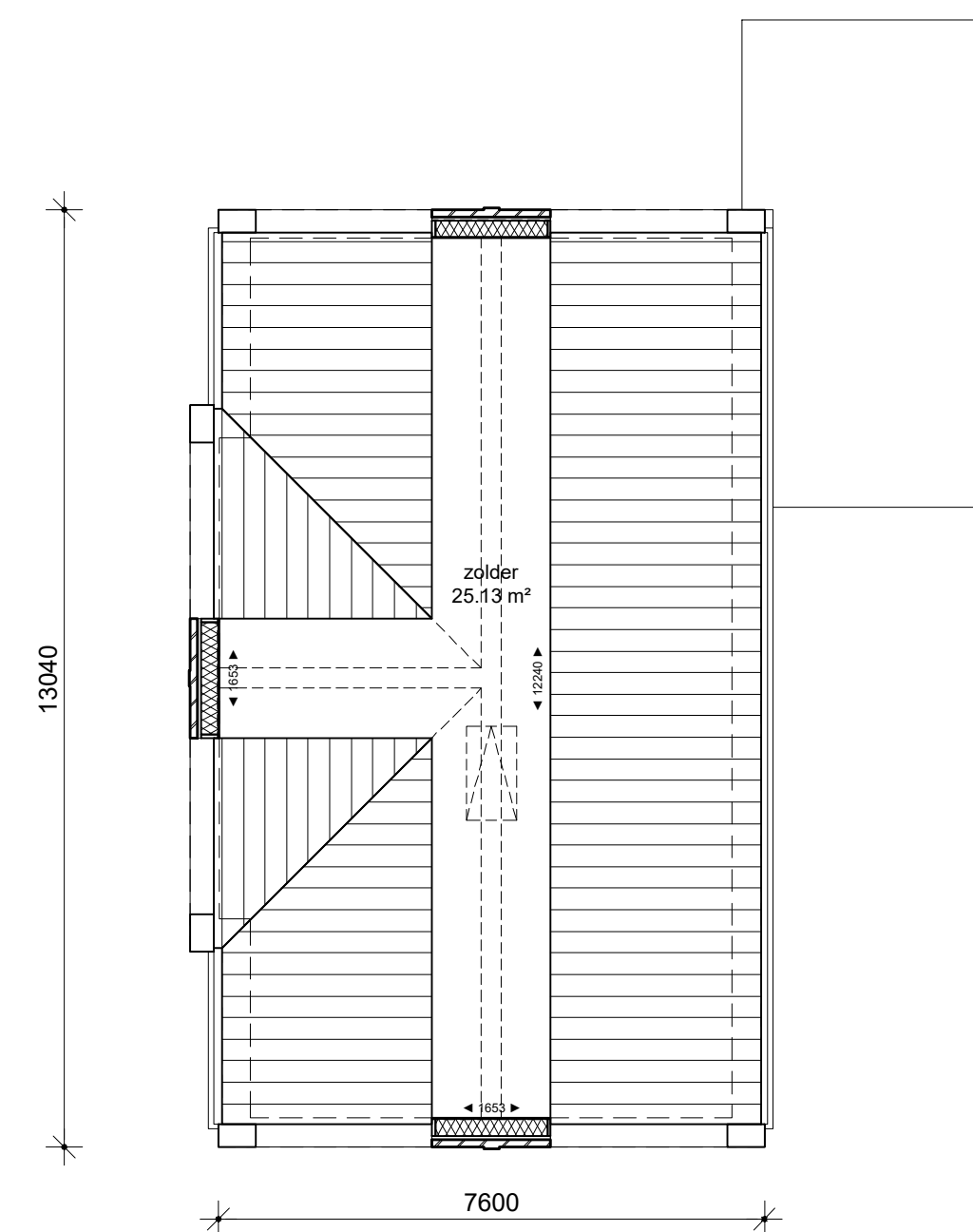
zolder
